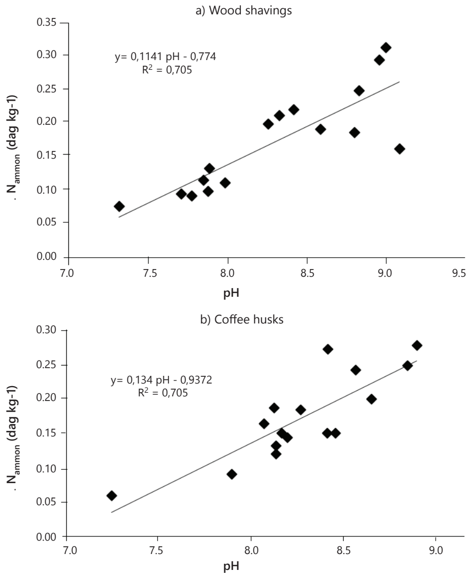
Figure 7. N_{\text{ammon}} values as a function of the pH: a) wood shavings; b) coffee husks.
