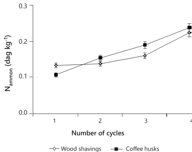
Figure 6. Concentrations of N ammon as a function of the number of cycles of wood shavings and coffee husks.
