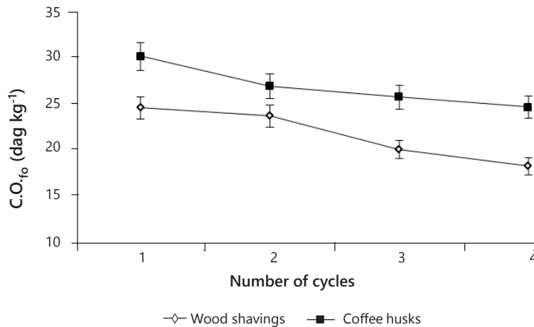
Figure 4. Values of total organic carbon ( C.O._{f0} ) in relation to the number of cycles of wood shavings and coffee husks.
