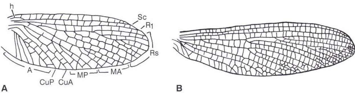
Fig. 6 - Wings of fossil Ephemeroptera: A) Misthodotes edmundsi Carpenter, Lower Permian (after Kinzelbach & Lutz 1984); B) Litopblebia oplata Riek, Upper Triassic (after Riek 1976).
